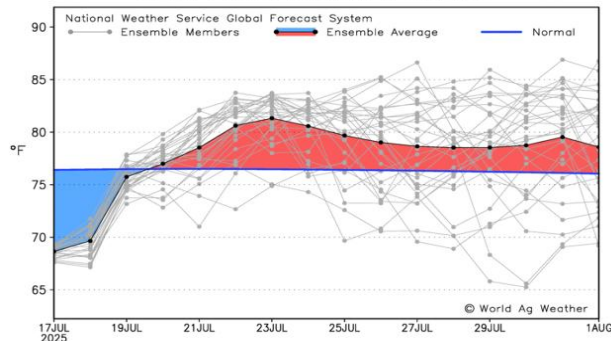
US Corn Temperature Forecast Daily-Mean Temperature Compared to Normal (°F) Production-Weighted Area Average 15-Day Forecast Beginning 17 July 2025
