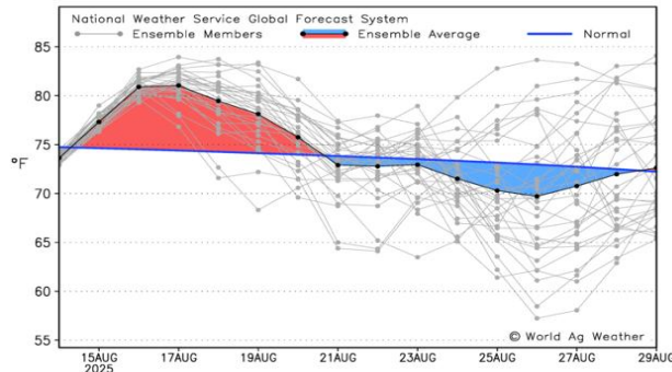
US Corn Temperature Forecast Daily-Mean Temperature Compared to Normal (°F) Production-Weighted Area Average 15-Day Forecast Beginning 14 August 2025
